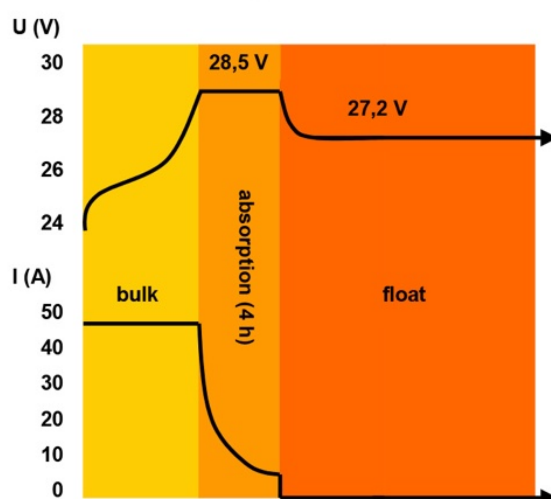
Charge curve
